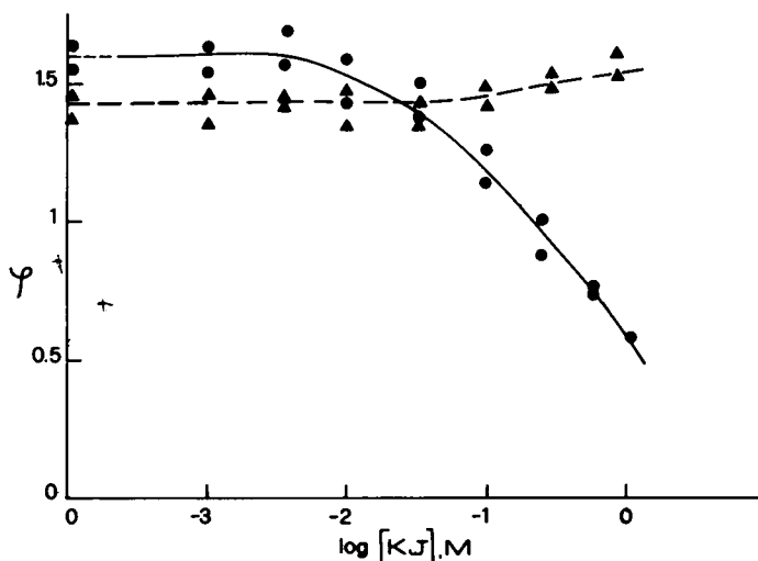
FIGURE 9 Effect of potassium iodide on the fluorescence of aqueous solutions of filipin (2.5 \mu M; excitation at 355 nm, emission at 480 nm: ●—●) and of erythrocyte ghosts-bound lucensomycin (2 \mu M lucensomycin + 200 \mu M membrane cholesterol; excitation at 307 nm, emission at 410 nm: ▲—▲).
